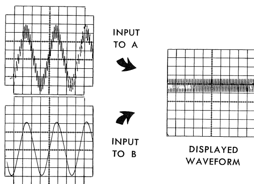
Fig. 3-2. Rejection of a common mode signal by the differential amplifier.
