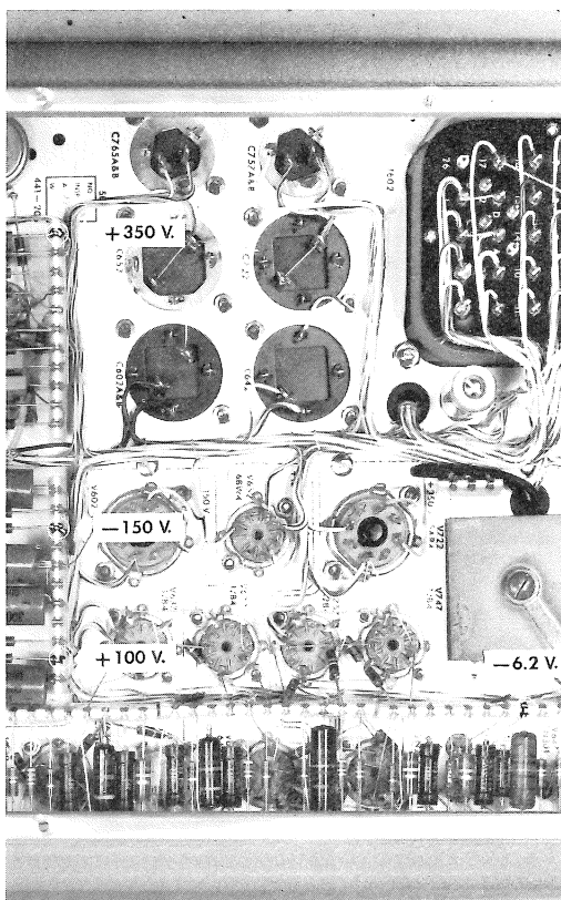
Fig. 5-4. Low voltage power supply test points.
