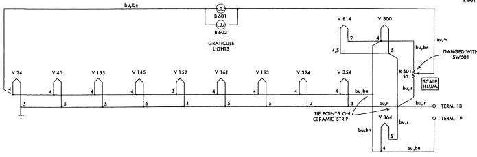
SWEEP CHASSIS
