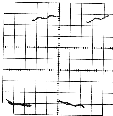
Fig. 6-10. Adjustment of the FEEDBACK BAL control. The waveform shown is typical of the waveforms obtained when the FEEDBACK BAL control is adjusted properly. The vertical amplifier is shielded by a small metal plate to reduce the noise level. Note that it is not usually possible to completely eliminate distortion of the square wave. The adjustment is made for minimum distortion.
